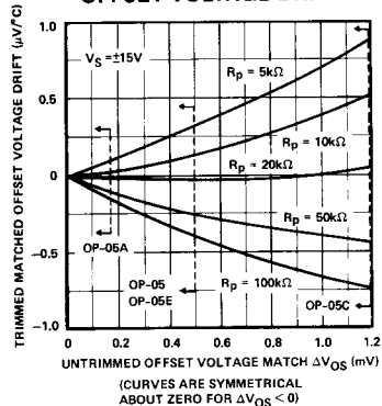
TRIMMED OFFSET VOLTAGE DRIFT
