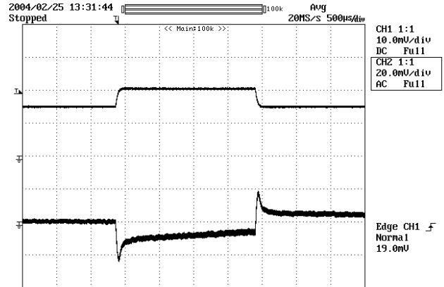
Figure 18 - Transient Response, 57 VDC, 75-100-75% Load Step. Top: Load Current, 1 A / div. Bottom: Output Voltage, 20 mV, 500 μs / div.
