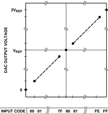
Figure 26. DAC Transfer Function
