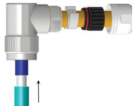
Step 6: Side heat shrink tubing onto cable
