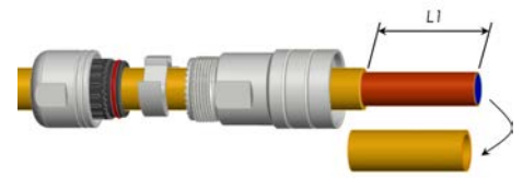
Step 2: Strip jacket
