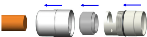
Step 1: Side components onto cable
