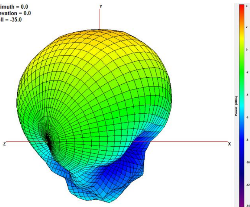
XZ Plane
