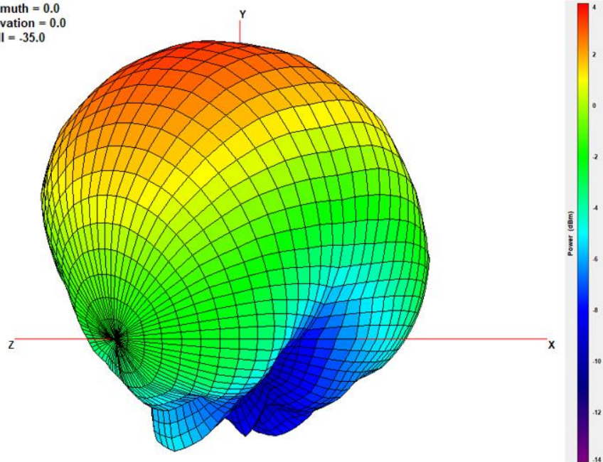
XZ Plane
