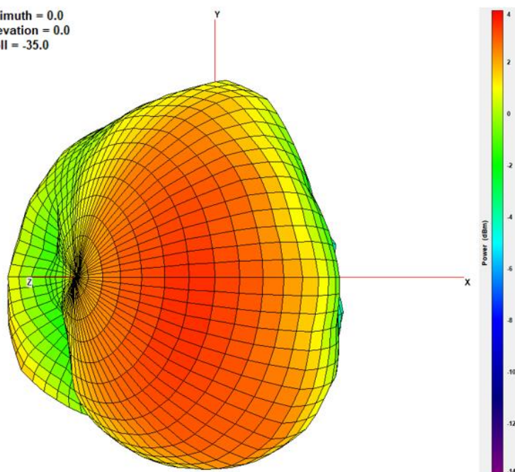
XZ Plane
