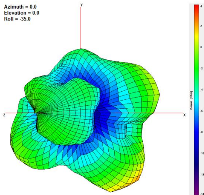
XZ Plane
