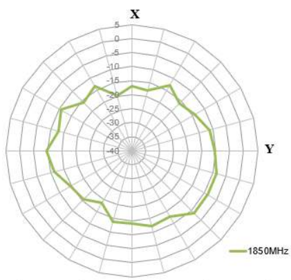
XY Plane
