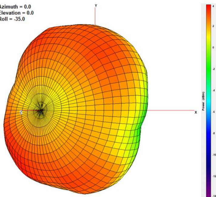
XZ Plane
