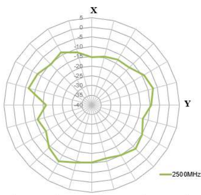
XY Plane
