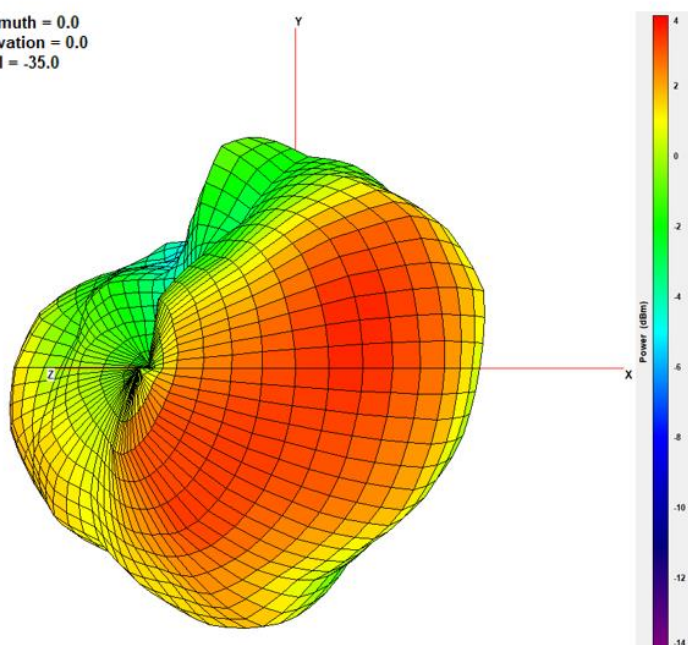
XZ Plane
