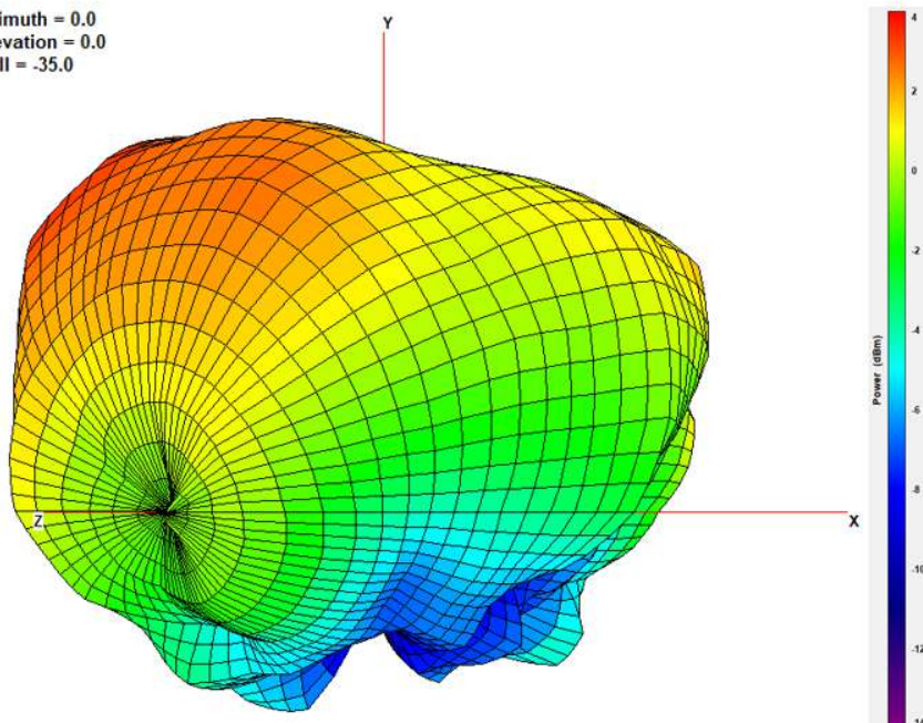
XZ Plane
