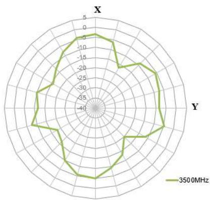
XY Plane
