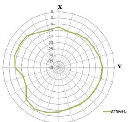
XY Plane
