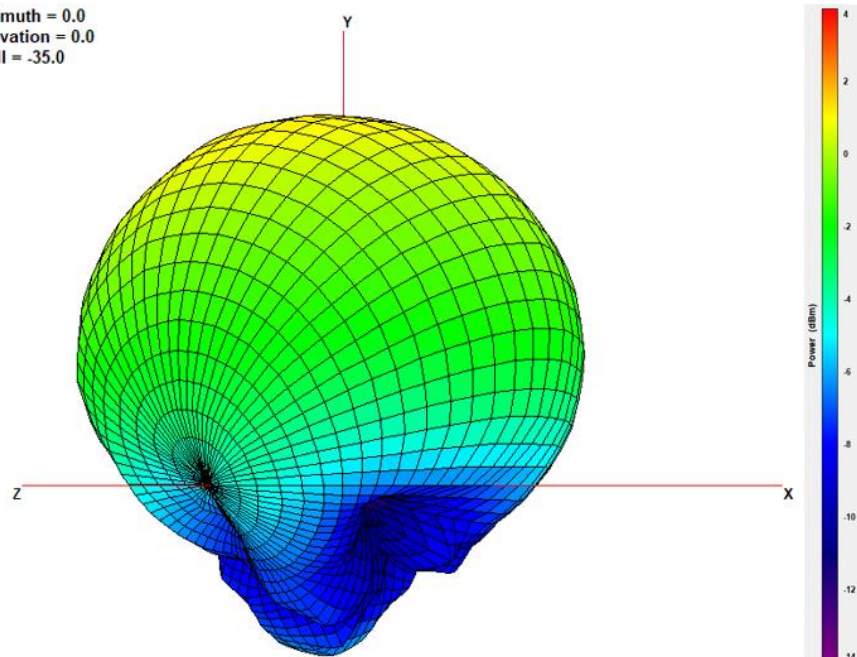
XZ Plane
