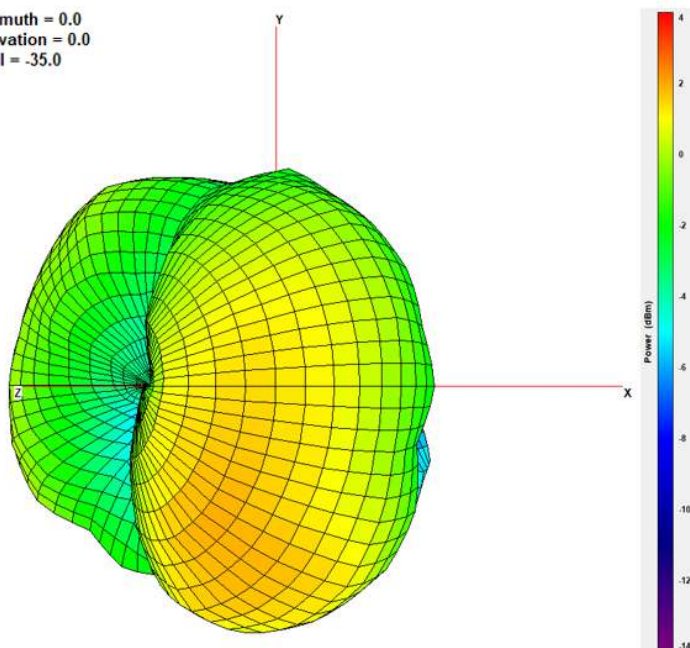
XZ Plane
