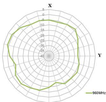
XY Plane
