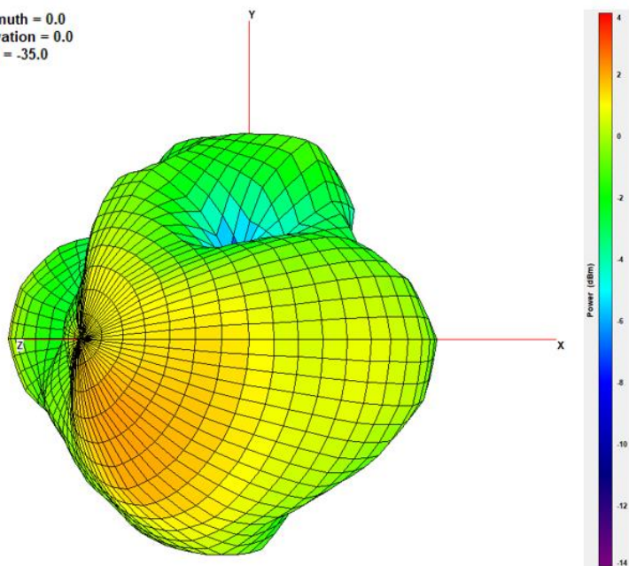
XZ Plane
