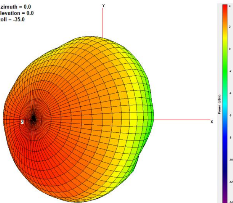
XZ Plane
