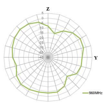
YZ Plane
