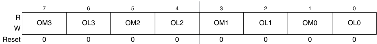
Figure 14-12. Timer Control Register 2 (TCTL2)
