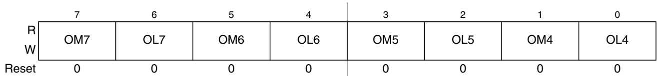
Figure 14-11. Timer Control Register 1 (TCTL1)
