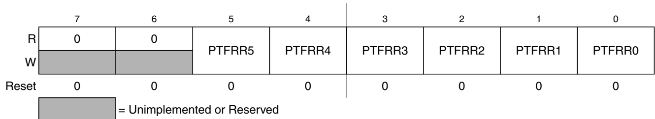
Figure 2-106. Port F Routing Register (PTFRR)
