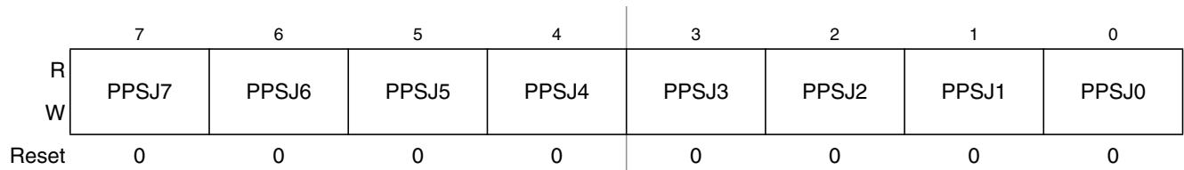
Figure 2-64. Port J Polarity Select Register (PPSJ)
