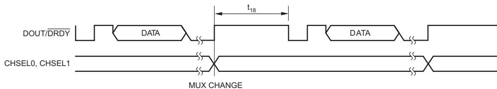
Figure 32. Multiplexer Operation
