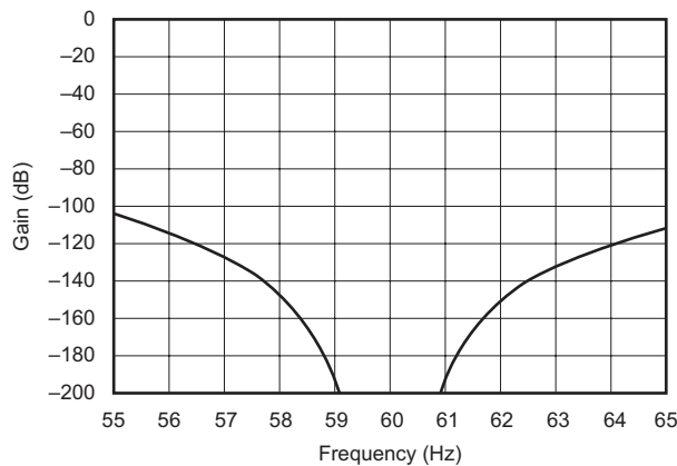
Figure 29. Expanded Digital Filter Response (60 Hz With a 60-Hz Data Output Rate)
