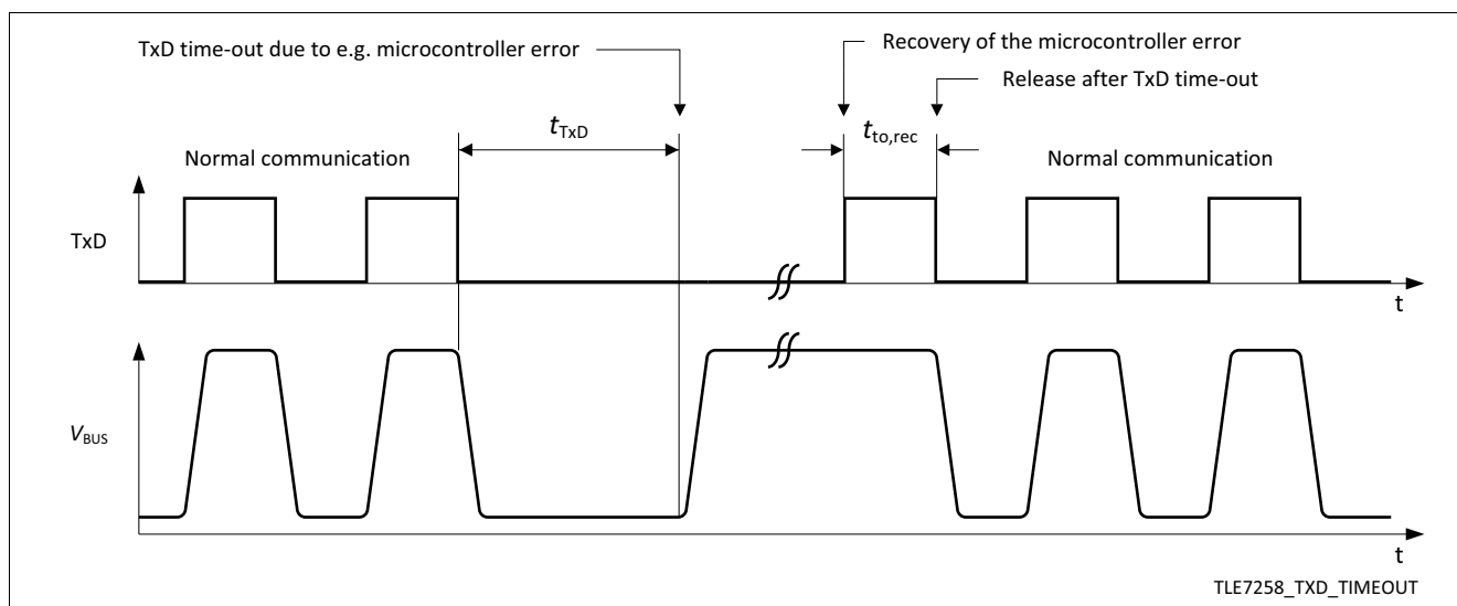
Figure 13 TxD time-out
