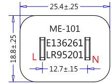
ME-101 (1-15P, Non-Polarized) (Dimensions of Plug Face)
