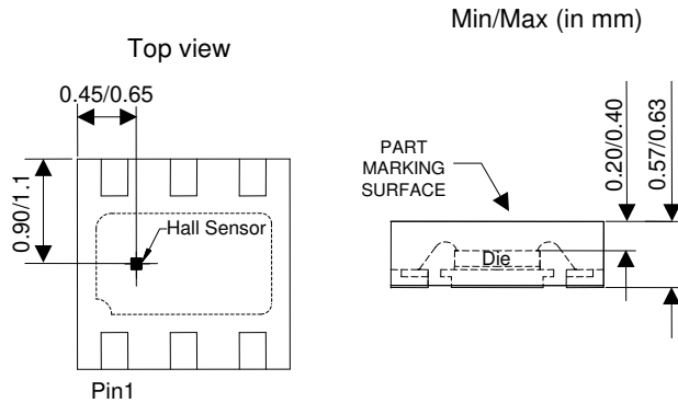
Sensor Location
