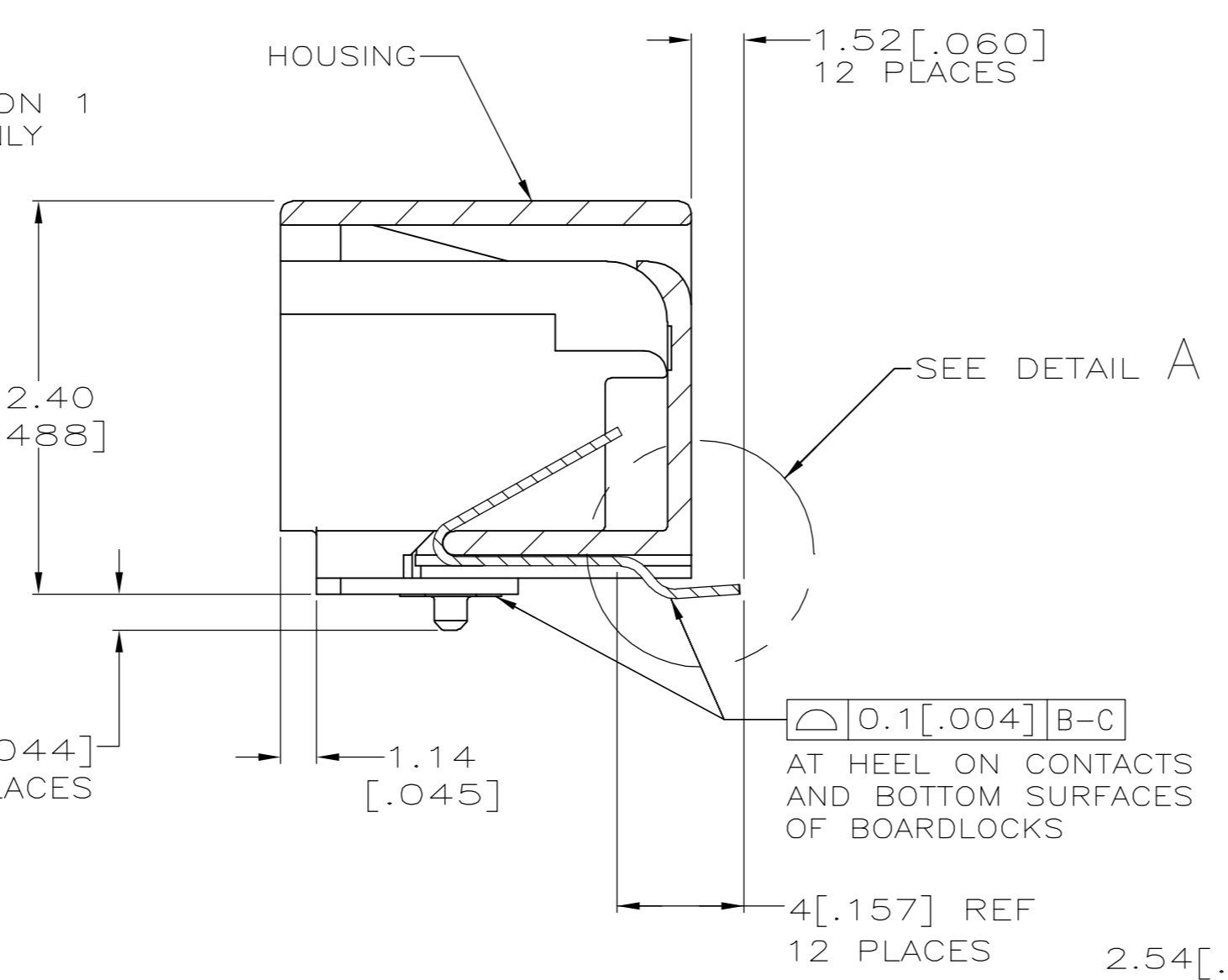
SECTION C-C
