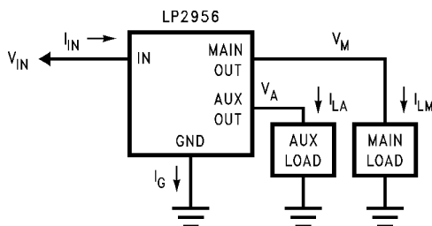
Figure 40. Current/Voltage Diagram
