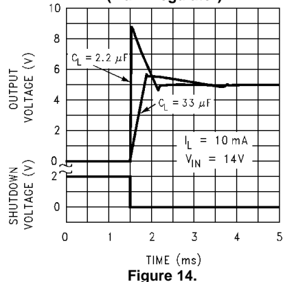
Enable Transient (Main Regulator)
