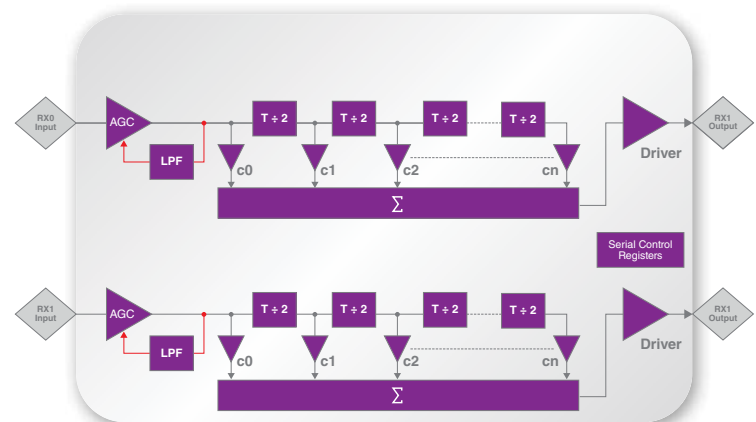
Functional Diagram
