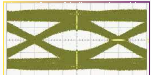
Equalized Output
