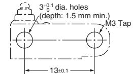
Mounting Hole Dimensions (Reference)
