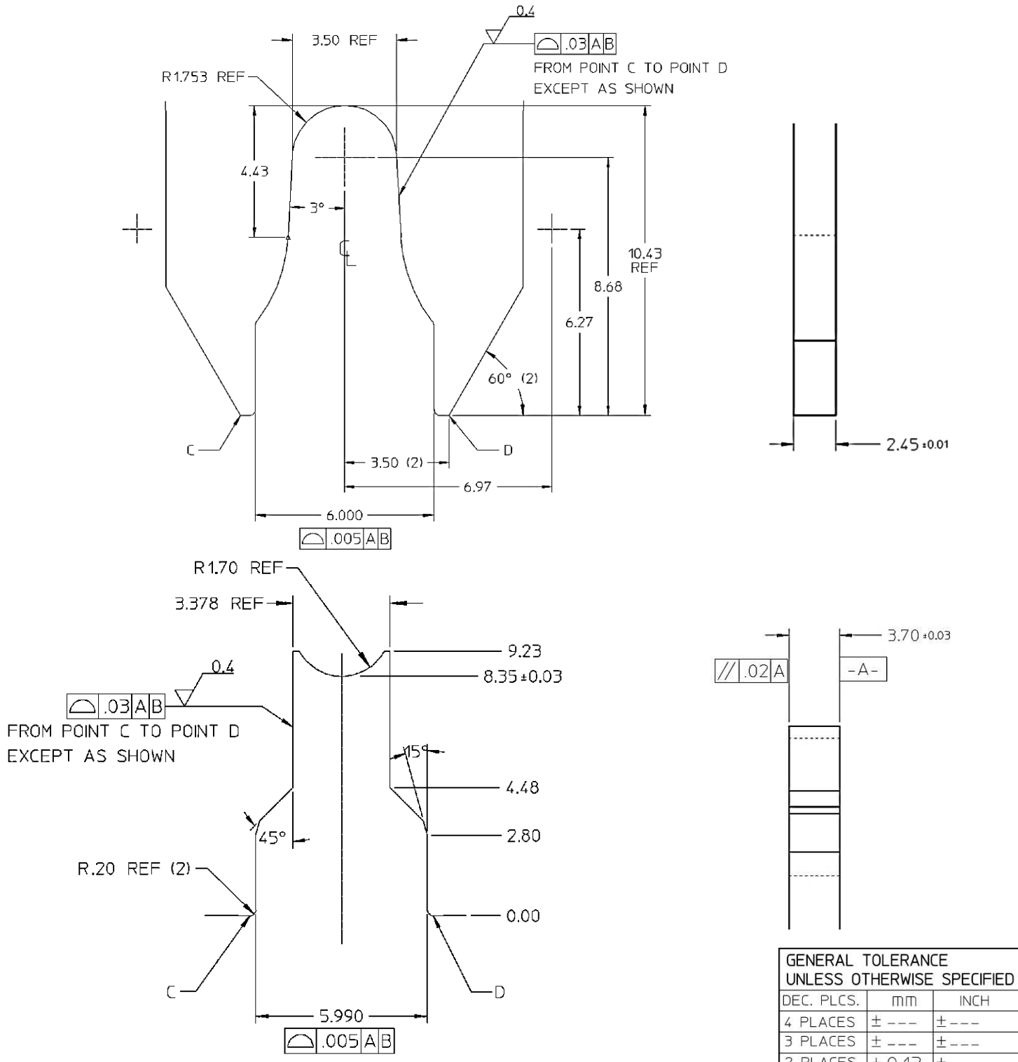
Figure 17 – Insulation Tooling Geometry (Grip Code 18 ONLY)
