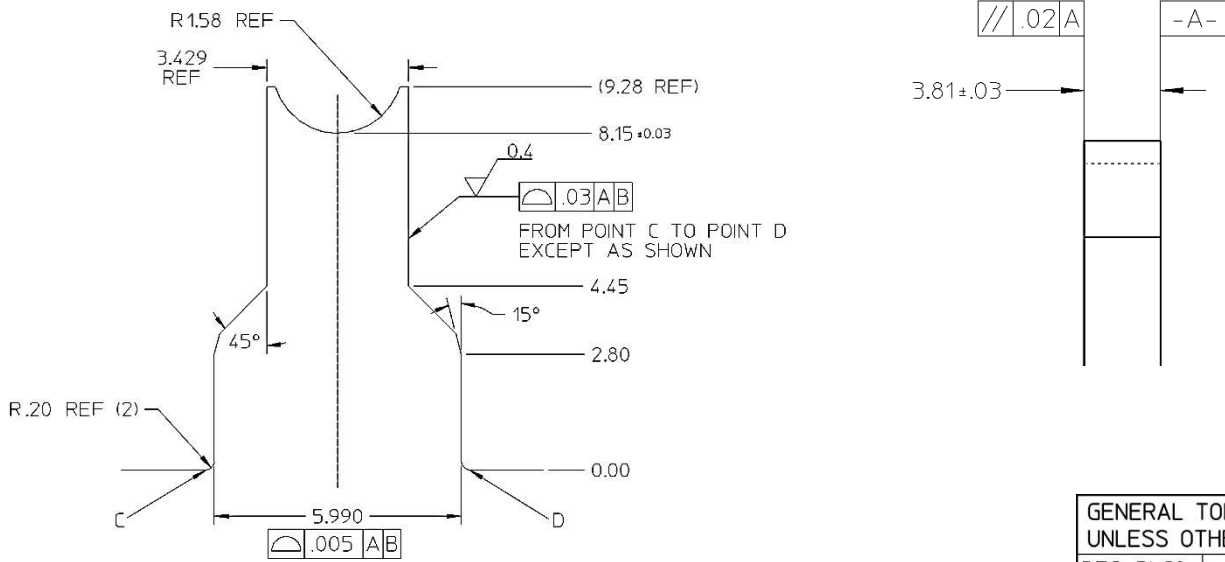
Figure 19 – Insulation Tooling Geometry (Grip Code 14 ONLY)
