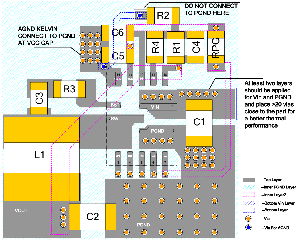
Figure 14: Recommend Layout
