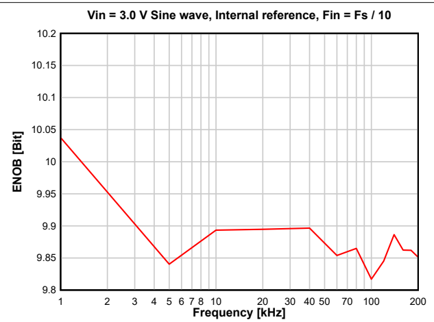
Figure 8-31. ENOB vs. Sampling Frequency
