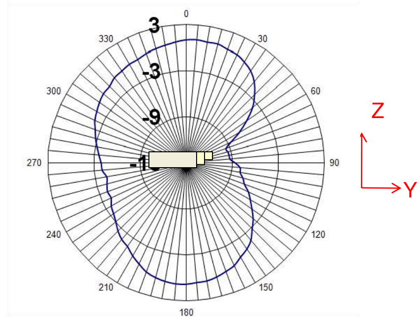
Figure 3d: Radiation diagram of Z-Y plane shows combined polarizations as measured on reference board
