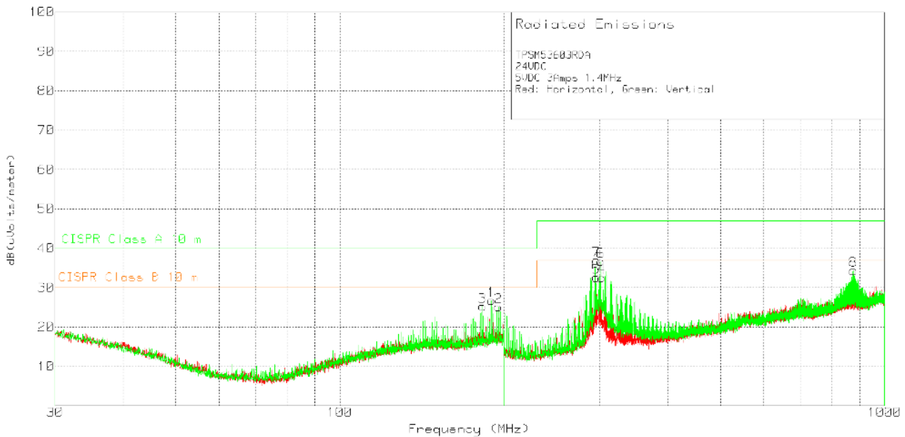
Figure 10-5. Radiated Emissions 24-V Input, 5-V Output, 3-A Load
