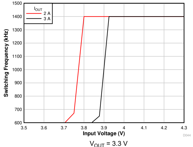
Figure 7-8. Frequency Foldback
