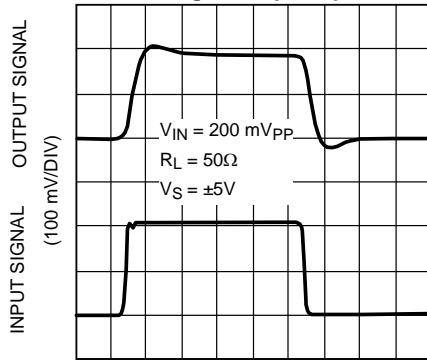
TIME (10 ns/DIV)
