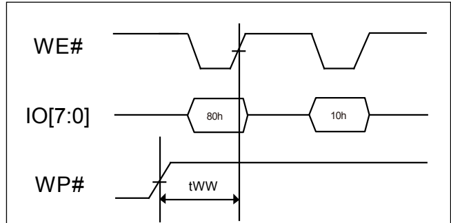
Figure 41-1. Enable Programming of WP# Signal
