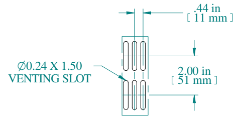
DETAIL A 2:1 TYPICAL
