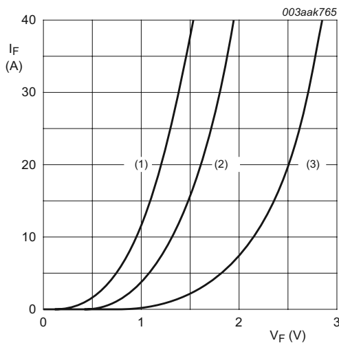
V_o = 1.311 \text{ V}; R_s = 0.015 \text{ } \Omega (1) T_j = 150 \text{ }^\circ\text{C} ; typical values (2) T_j = 150 \text{ }^\circ\text{C} ; maximum values (3) T_j = 25 \text{ }^\circ\text{C} ; maximum values
