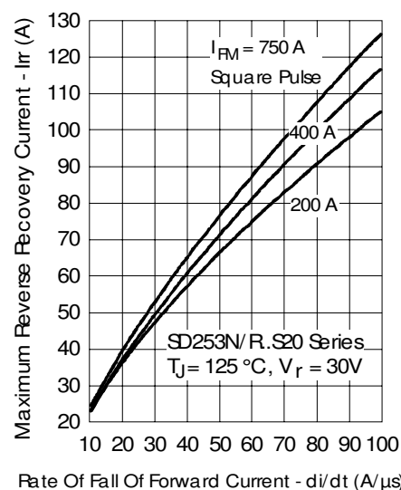
Fig. 14 - Recovery Current Characteristics
