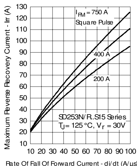
Fig. 11 - Recovery Current Characteristics
