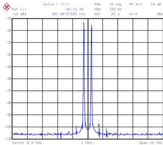
FIGURE 11. TWO TONES (CKHzF=6) AT 8.5MHz, 50MSPS CLOCK, 500kHz SPACING (82dBc - 10MHz WINDOW, 6dB PAD)
