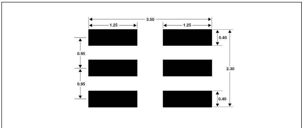
Figure 52: Suggested FN Package PCB Layout
