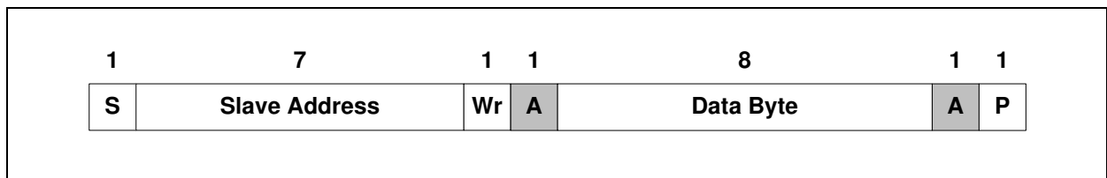
Figure 26: SMBus Send Byte Protocol
