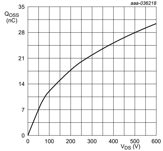
Fig. 7. Output charge as a function of drain-source voltage; typical values Freq. = 100 kHz
