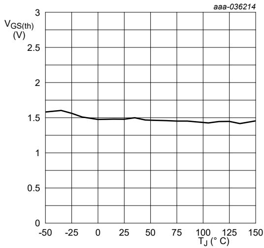
Fig. 8. Gate-source threshold voltage as a function of junction temperature I_D = 12.2\text{ mA} ; V_{DS} = V_{GS}
