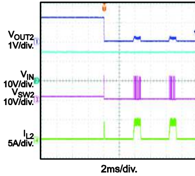
Short Circuits Entry (CH2) I_{OUT} = 0A
