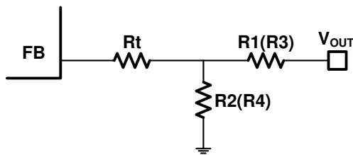
Figure 5: Feedback Network
