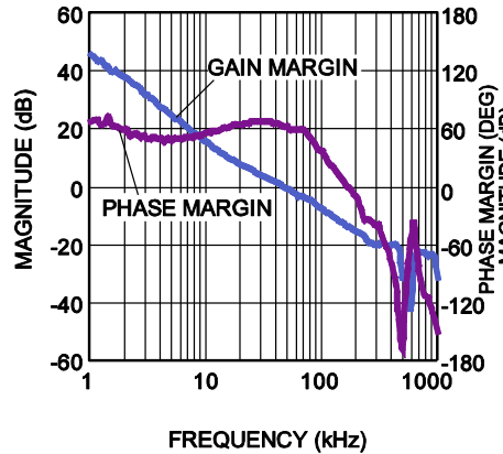
Bode Plot
