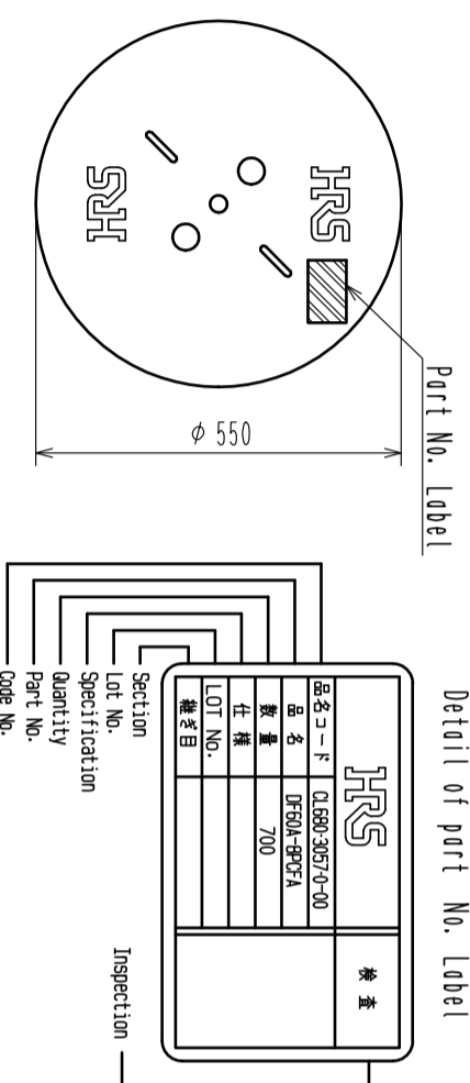
2 Style and Dimension of Reel
