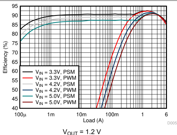
Figure 9-6. Efficiency
