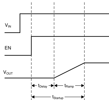
Figure 8-1. Start-up Sequence
