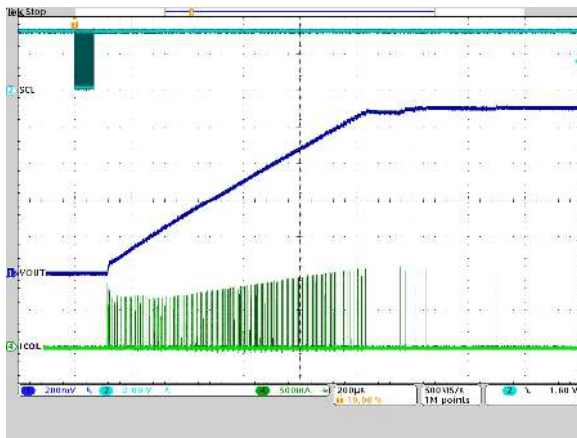
Figure 9-14. Forced PWM Operation
