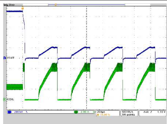
Figure 9-19. HICCU Protection
