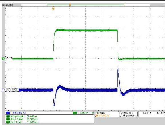
Figure 9-16. Start-up by Software Enable Device Bit
