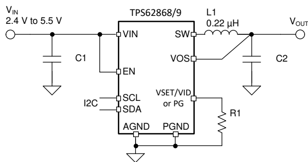
Figure 9-1. Typical Application
