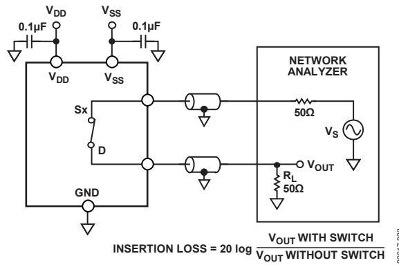
Figure 32. Bandwidth
