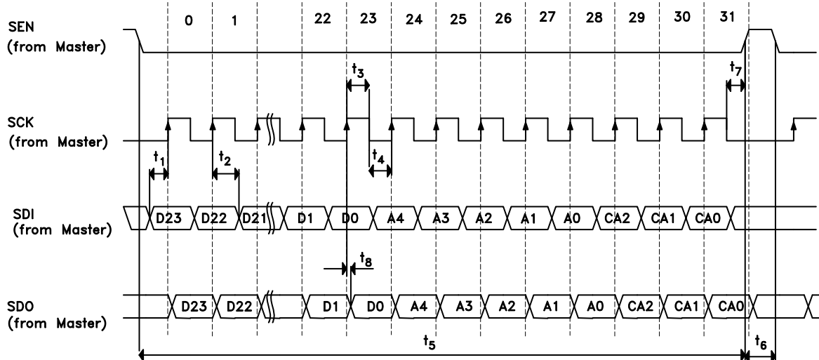
Figure 38. SPI Timing Diagram
