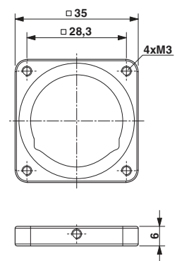
Dimensioned drawing
