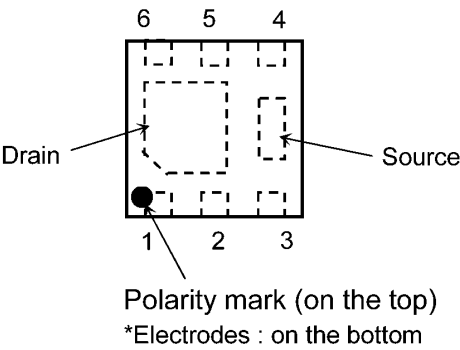
Fig. 6.2 Pin Condition (Top View)
