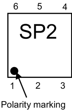
Fig. 6.1 Marking
