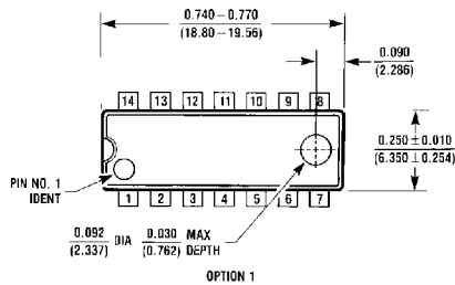
14-Lead Ceramic Dual-In-Line Package (J) Order Number DM54S30J Package Number J14A
