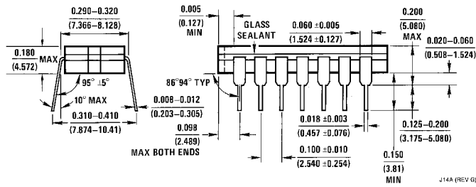
14-Lead Ceramic Dual-In-Line Package (J) Order Number DM54S30J Package Number J14A
