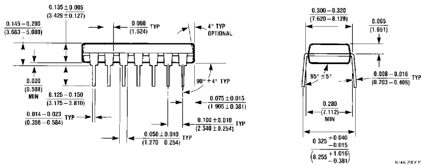
14-Lead Molded Dual-In-Line Package (N) Order Number DM74S30N Package Number N14A
