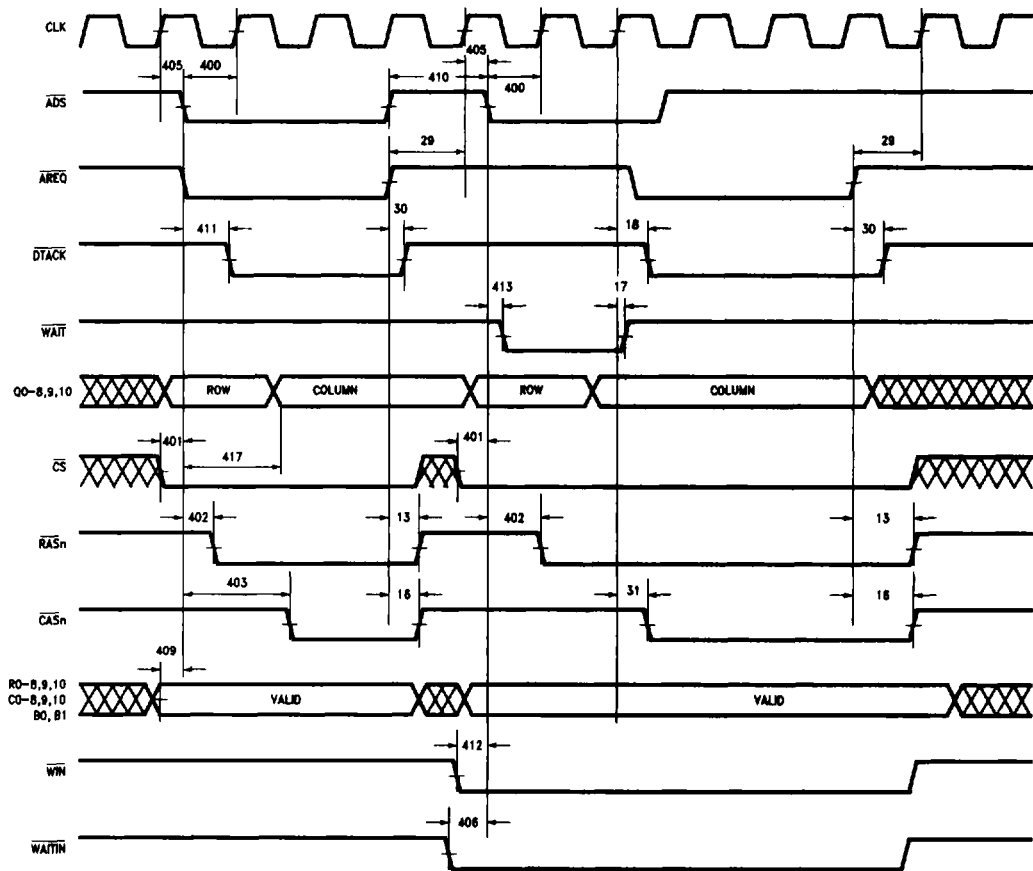
FIGURE 42. 400: Mode 1 Timing
