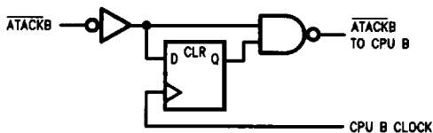
C. Synchronize \overline{ATACKB} to CPU B Clock. This is useful if CPU B runs asynchronous to the DP8422V, DP84T22.
