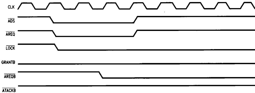
FIGURE 35. LOCK Function
