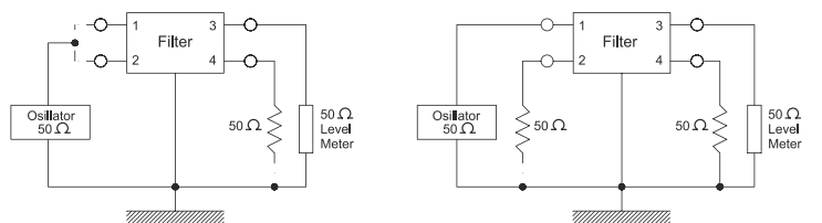
Common mode
