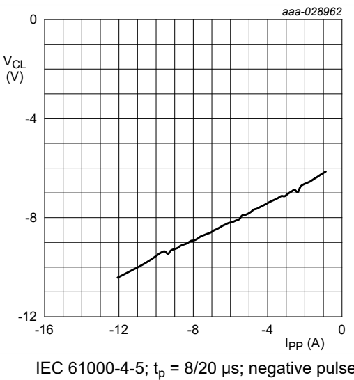
Fig. 9. Negative clamping voltage (8/20 \mu s pulse); typical values
