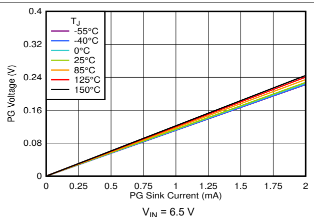
Figure 7-66. PG Voltage vs PG Current Sink
