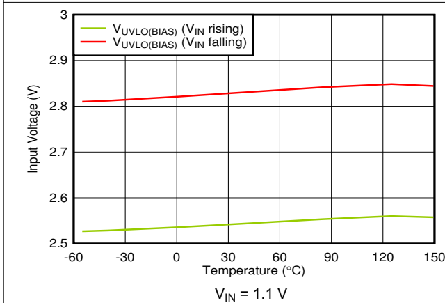
Figure 7-63. V_{BIAS} UVLO vs Temperature
