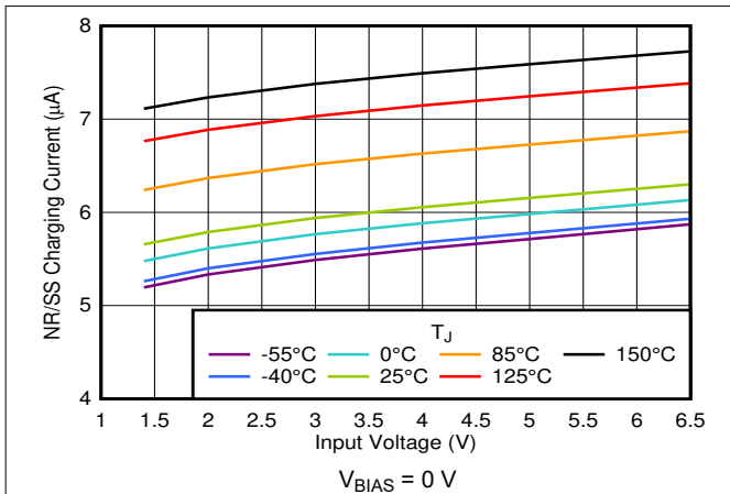
Figure 7-61. I_{NR/SS} Current vs Input Voltage
