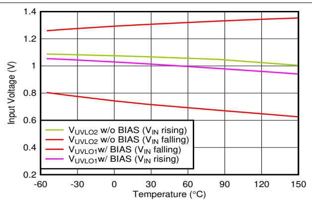
Figure 7-62. V_{IN} UVLO vs Temperature
