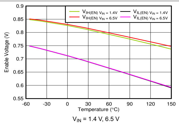
Figure 7-64. Enable Threshold vs Temperature
