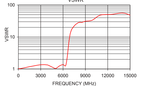
VLF-5850+ VSWR
