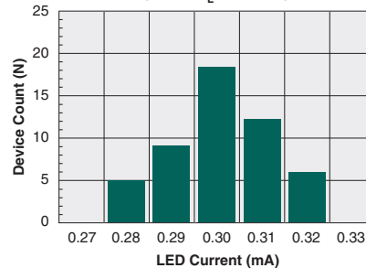
Typical I_f for Switch Dropout (N=50, I_L=120mA )
