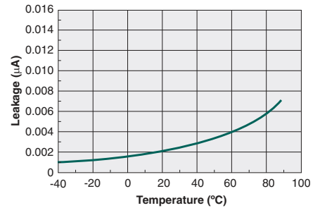
Typical Leakage vs. Temperature Measured Across Pins 3 & 4
