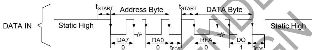
Figure 4. Single Wire Digital Dimming Timing, without Acknowledge RFA=0
