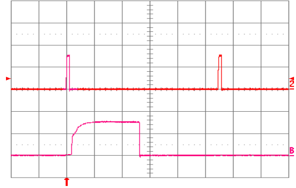
Fig. 2.5V.12: Load current (top trace, 20 A/div., 20 ms/div.) into a 10 m \Omega short circuit during restart, at V_{in} = 48 V. Bottom trace (20 A/div., 1 ms/div.) is an expansion of the on-time portion of the top trace.
