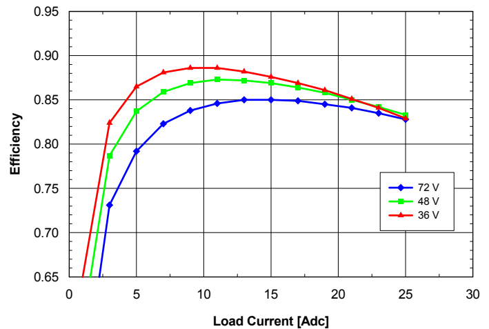
Fig. 1.8V.2: Efficiency vs. load current and input voltage for SQM48T/S25018 converter mounted vertically with air flowing from pin 3 to pin 1 at a rate of 300 LFM (1.5 m/s) and T_A = 25^\circ\text{C} .
