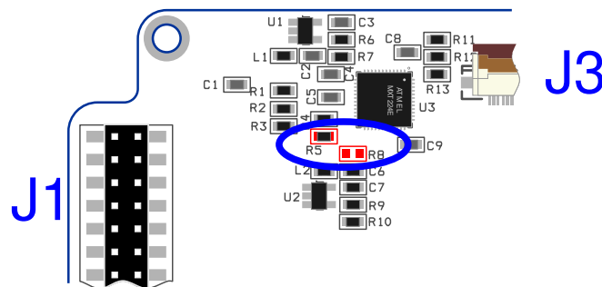
Figure 3 - Touch Controller I 2 C Address Selection
