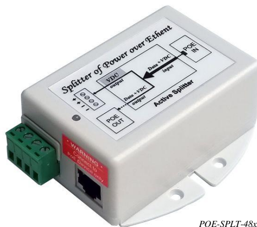
POE-SPLT-48xxG-P PoE Converter/Splitter with PoE passthru
