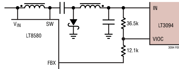
Figure 9. VIOC Connection Using LT8580
