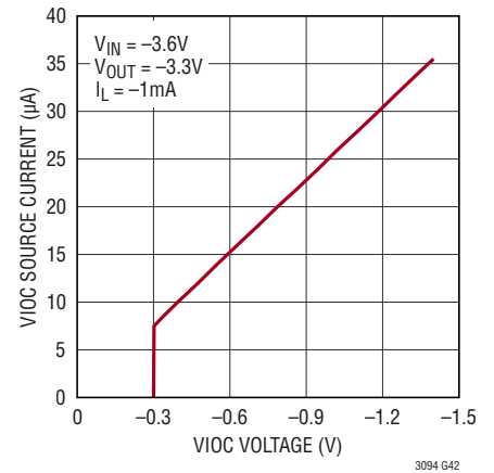
VIOC Source Current
