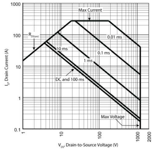
Figure 18 • Forward Safe Operating Area
