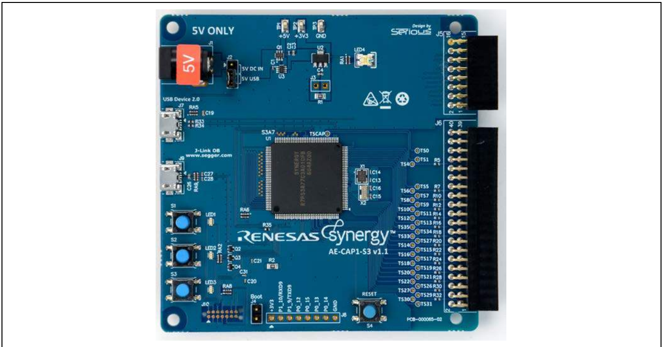
Figure 2 AE-CAP1-S3 Target Board
