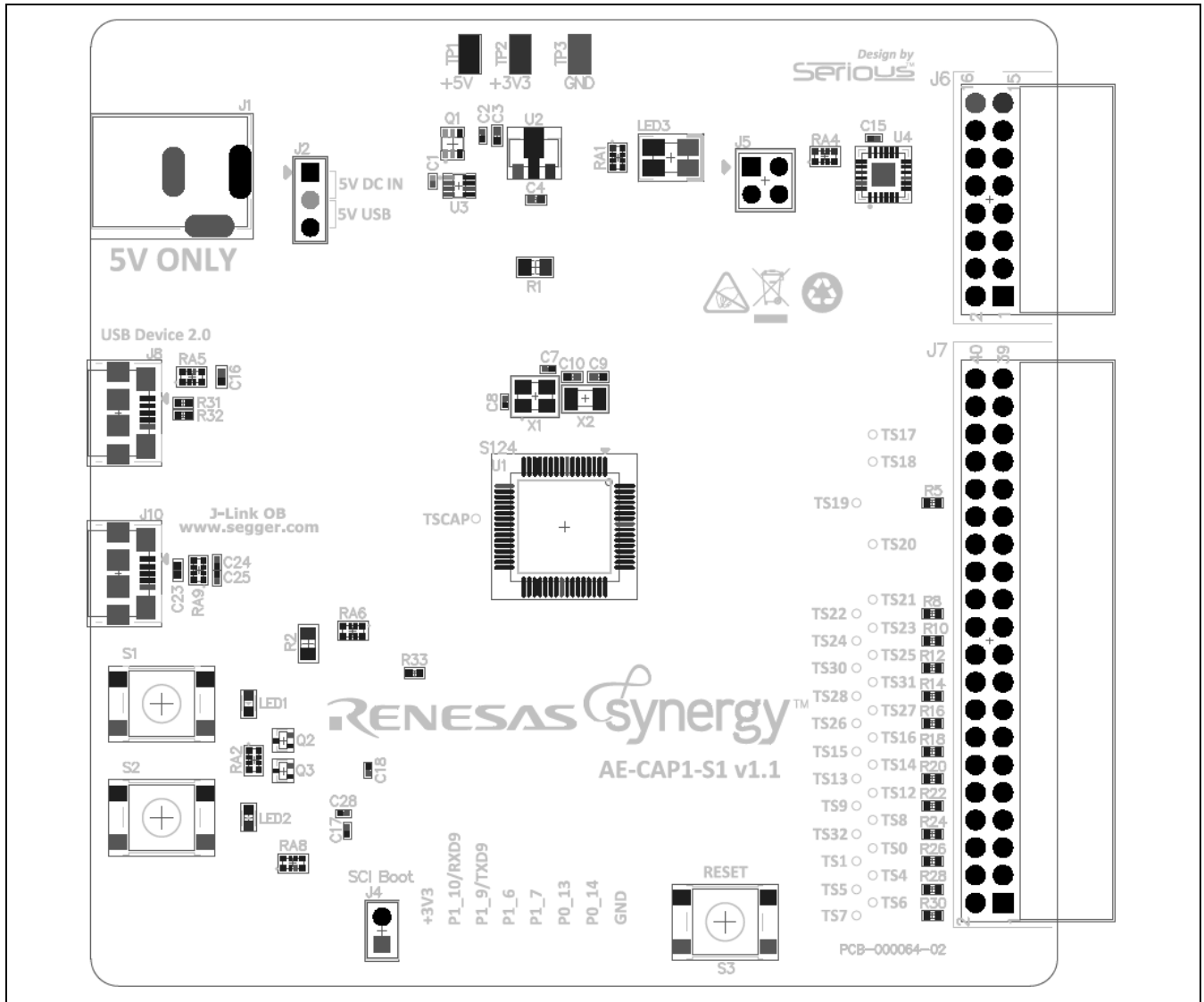
Figure 7 AE-CAP1-S1 Target Board Overall Component Placement, Top
