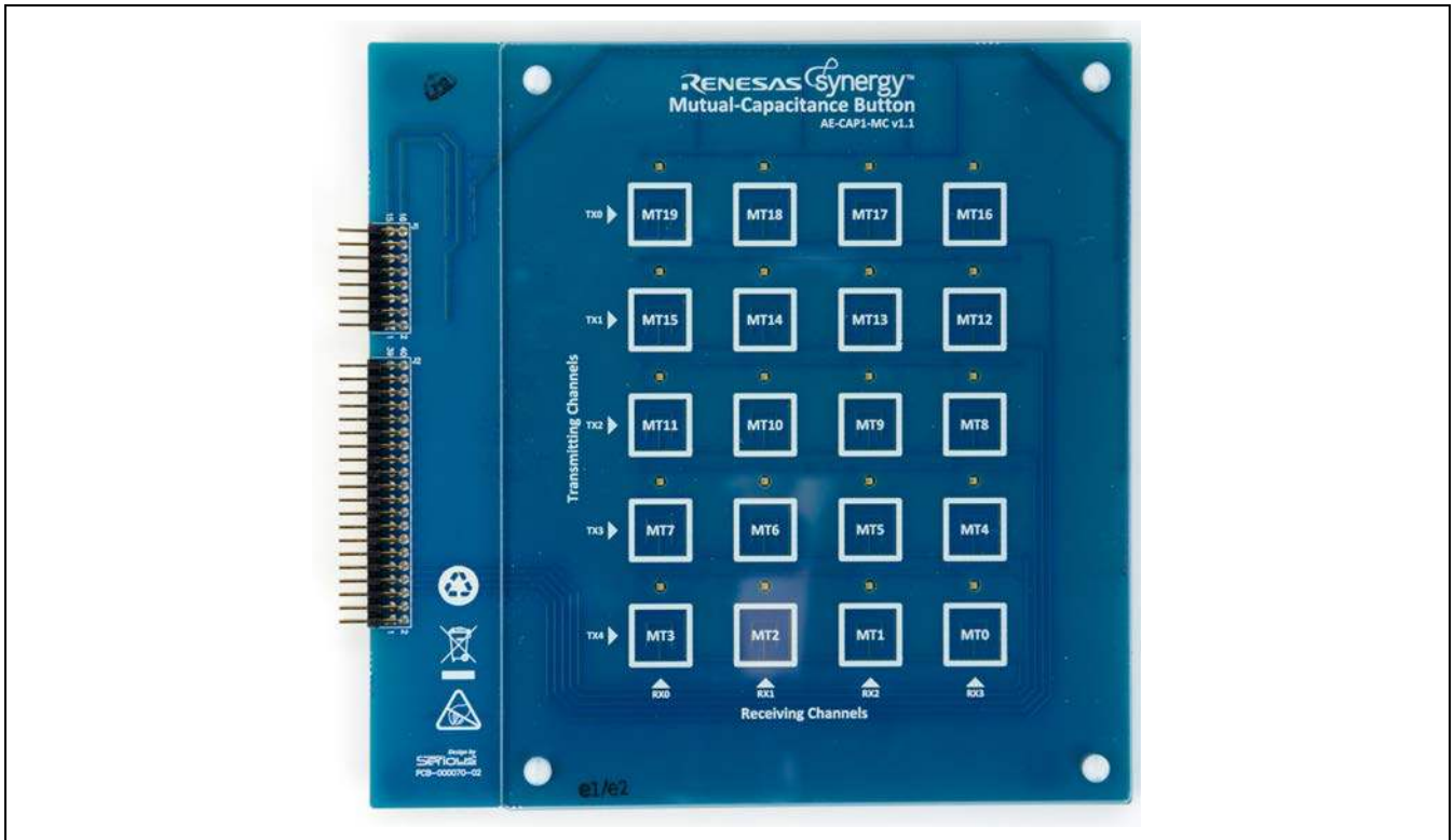
Figure 4 AE-CAP1-MC Application Board
