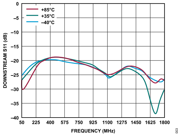
Figure 3. Downstream S11 vs. Frequency Over Temperature, V_{DD} = 8.0\text{ V}
