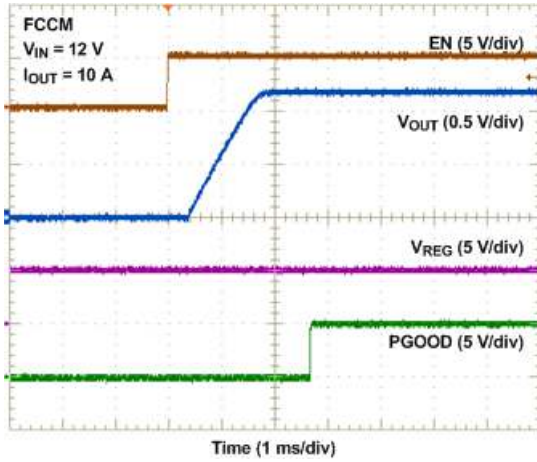
Figure 9-2. Start-Up
